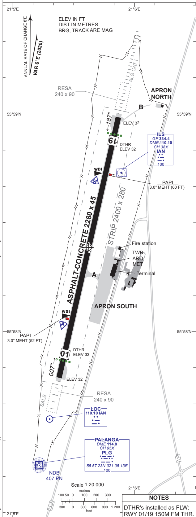
RWY MARKING AIDS
